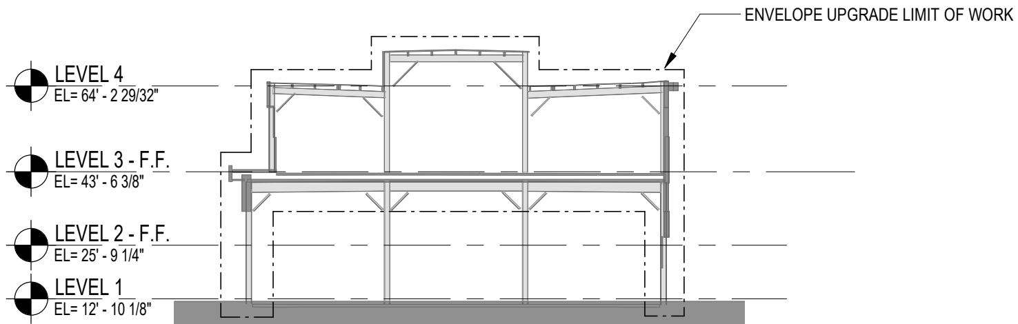
3 BUILDING SECTION - ENVELOPE UPGRADE LIMIT OF WORK SCALE: 1/32" = 1'-0"
