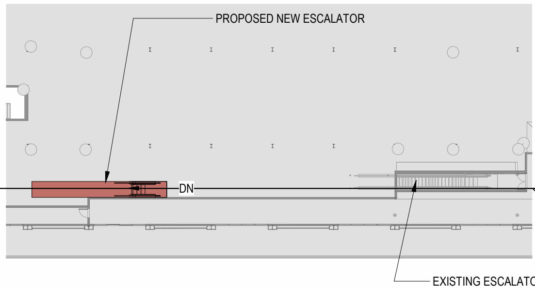
2 PARTIAL LEVEL 3 - ESCALATOR SCALE: 1/32" = 1'-0"
