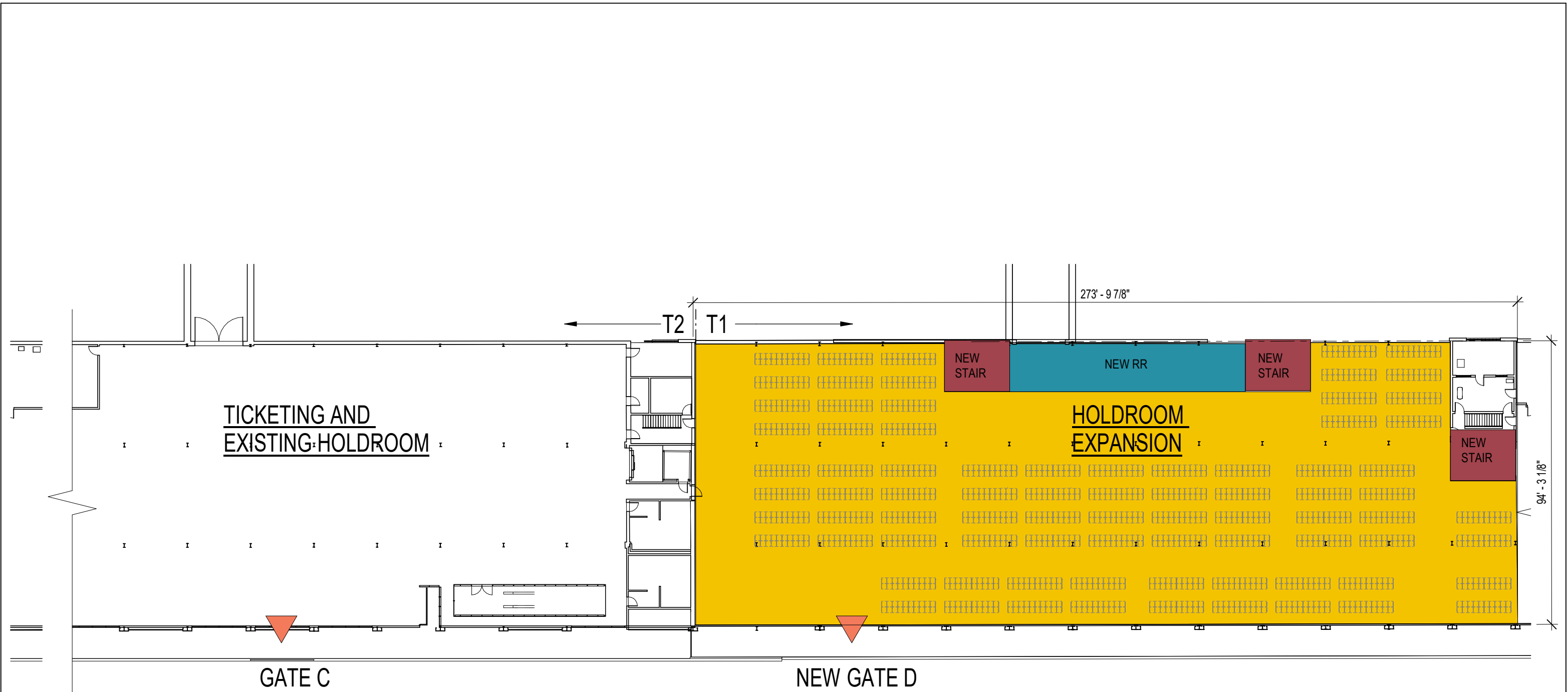
1 LEVEL 3 - HOLDROOM EXPANSION SCALE: 1/32" = 1'-0"
