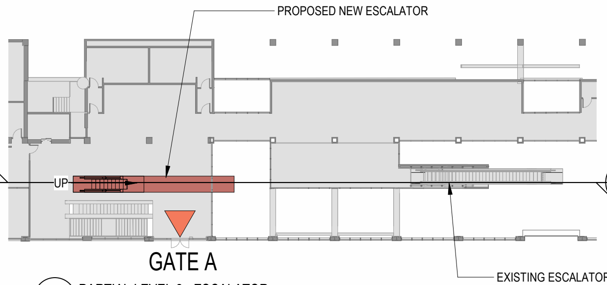
1 PARTIAL LEVEL 2 - ESCALATOR SCALE: 1/32" = 1'-0"
