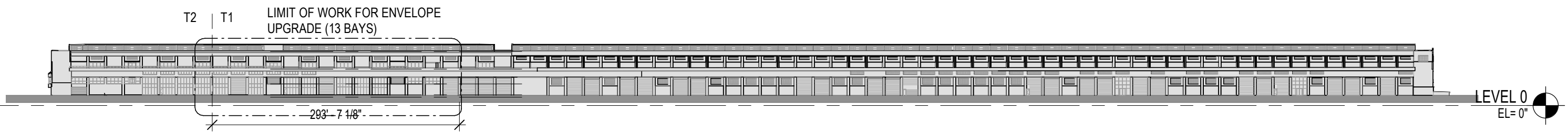
2 EXTERIOR ELEVATION PIER SIDE ENVELOPE UPGRADE LIMIT OF WORK SCALE: 1" = 120'-0"
