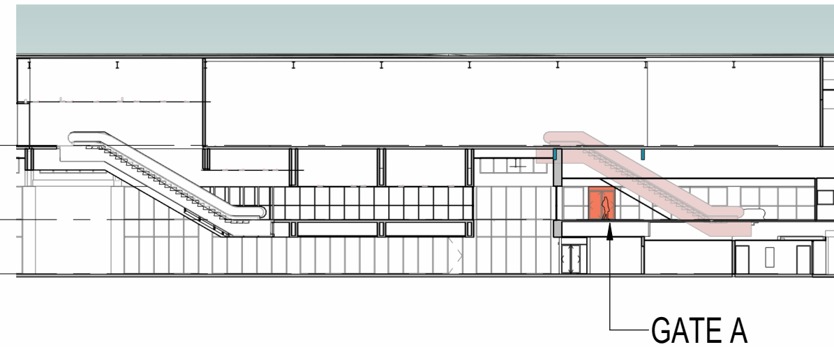
4 PARTIAL SECTION - LOOKING TOWARD SEA SCALE: 1/32" = 1'-0"
