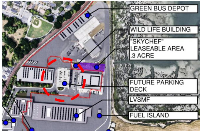
PARKING DECK SITE PLAN
