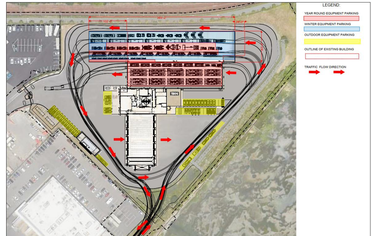
PROPOSED FLOOR PLAN AND SECTION OF THE NEW BAY
