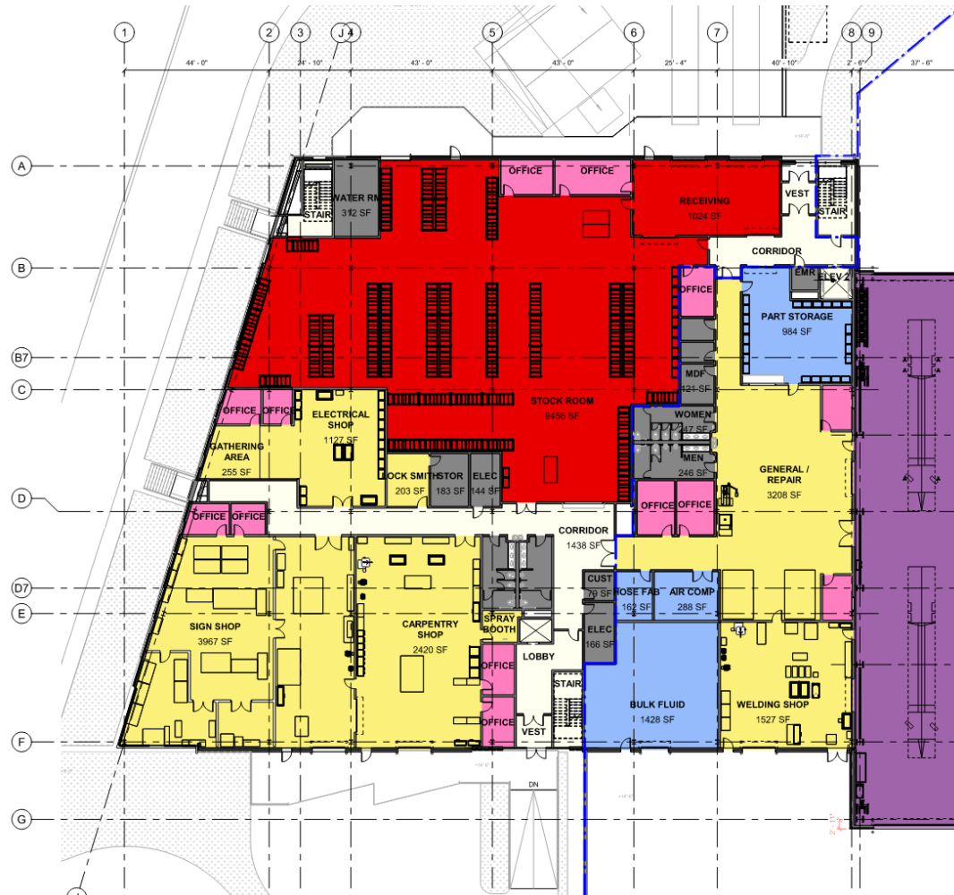
ENLARGED FIRST FLOOR PLAN | WORKSHOPS
