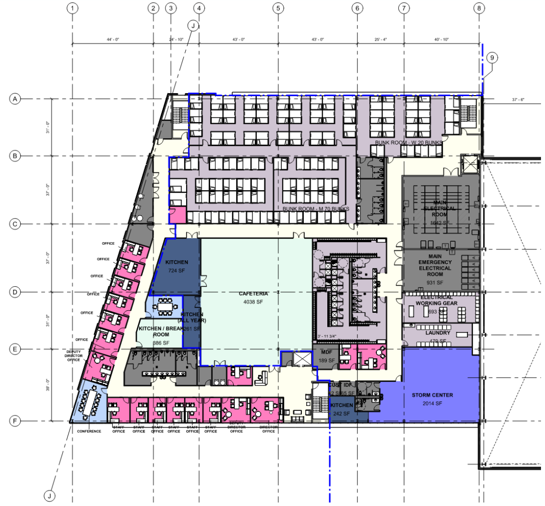
ENLARGED SECOND FLOOR PLAN | BUNKS
