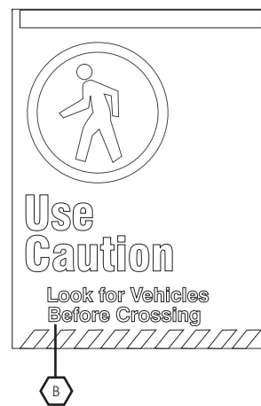
SIGN FACE ALTERNATE LAYOUT Scale: 3/4" = 1'-0"
