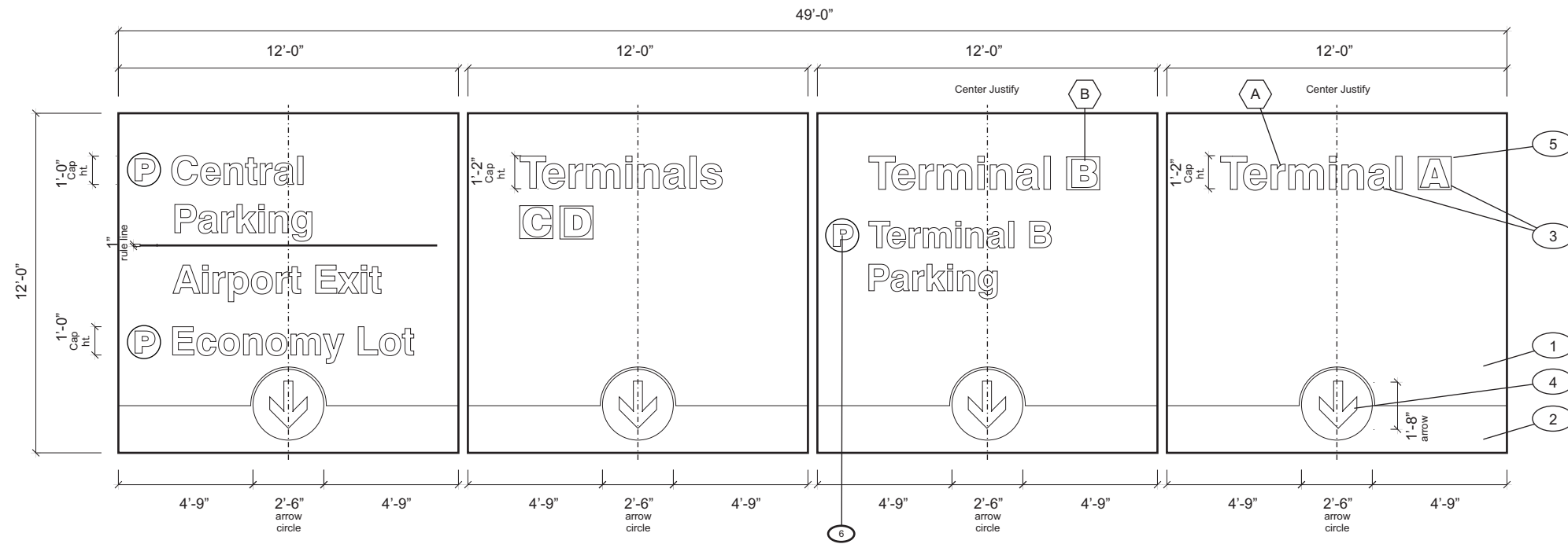
SIGN FACE LAYOUT Scale: 3/16" = 1'-0"
