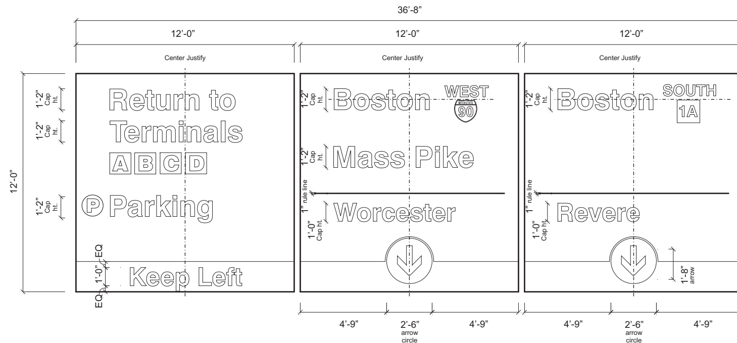
SIGN FACE ALTERNATE LAYOUT - B
