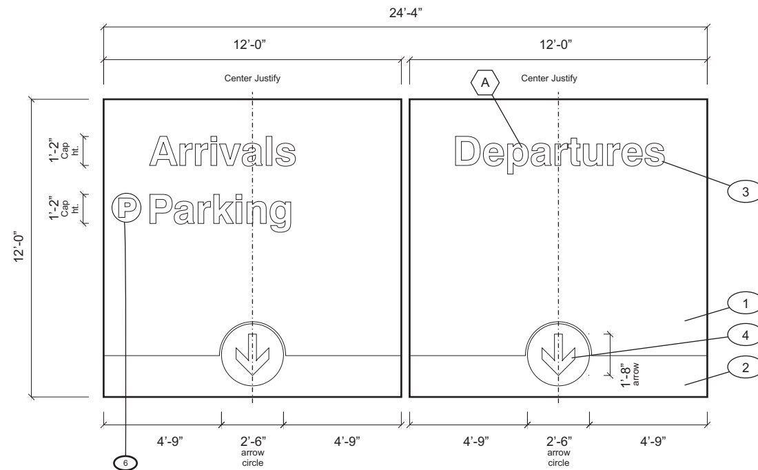
SIGN FACE LAYOUT
