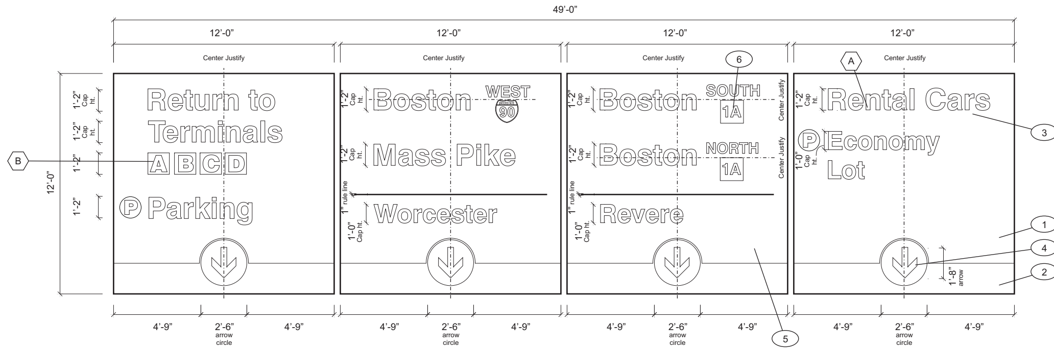
SIGN FACE ALTERNATE LAYOUT - A
