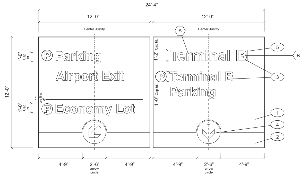
SIGN FACE LAYOUT Scale: 3/16" = 1'-0"
