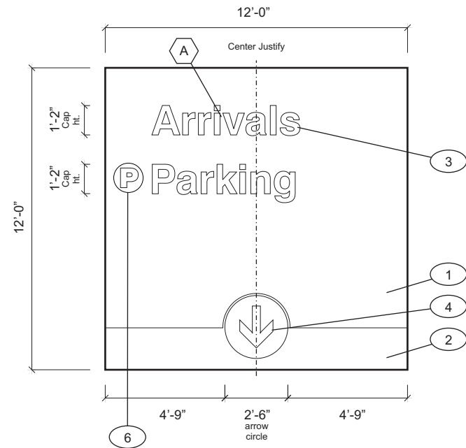
SIGN FACE LAYOUT Scale: 3/16" = 1'-0"
