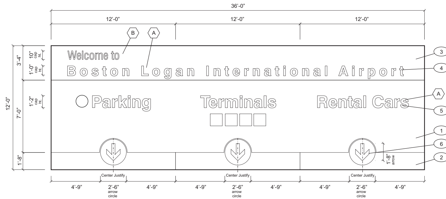
SIGN FACE LAYOUT Scale: 3/16" = 1'-0"
