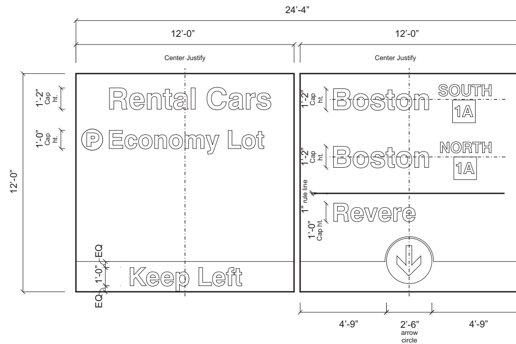
SIGN FACE ALTERNATE LAYOUT - B
