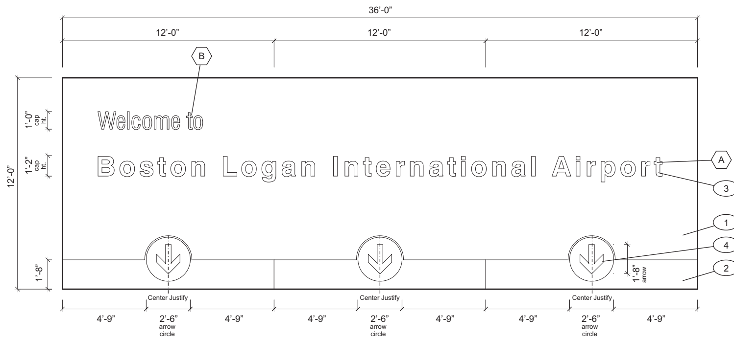
SIGN FACE LAYOUT - ALTERNATE LAYOUT
