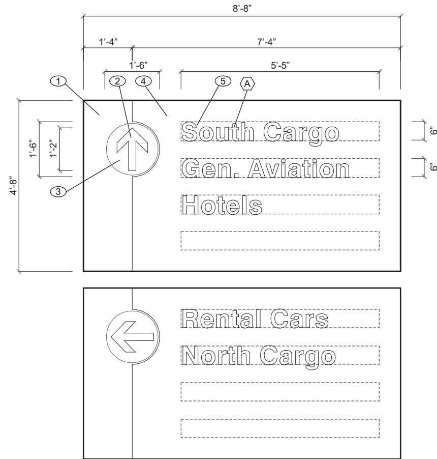
SIGN FACE LAYOUT Scale: 3/16" = 1'-0"
