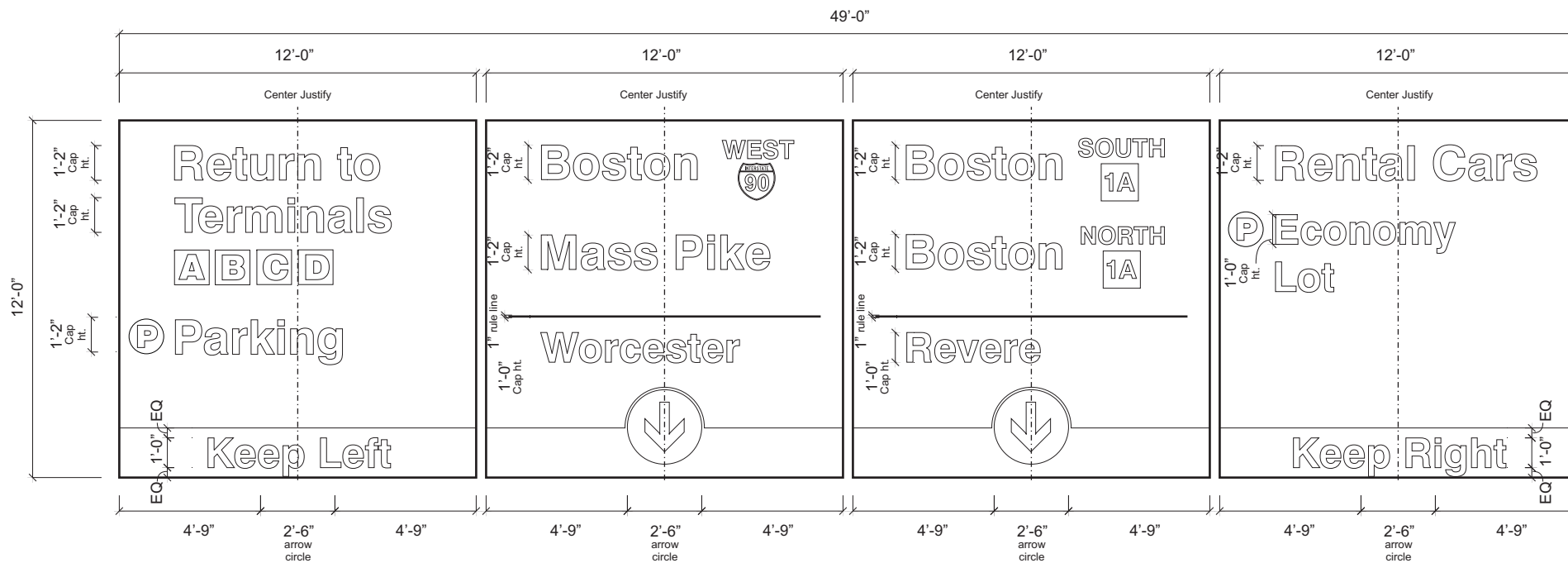
SIGN FACE ALTERNATE LAYOUT - B
