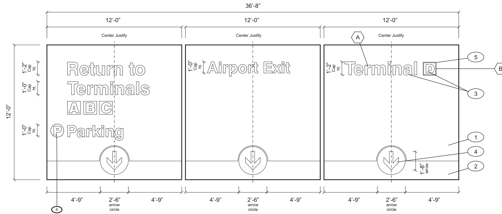
SIGN FACE LAYOUT Scale: 3/16" = 1'-0"
