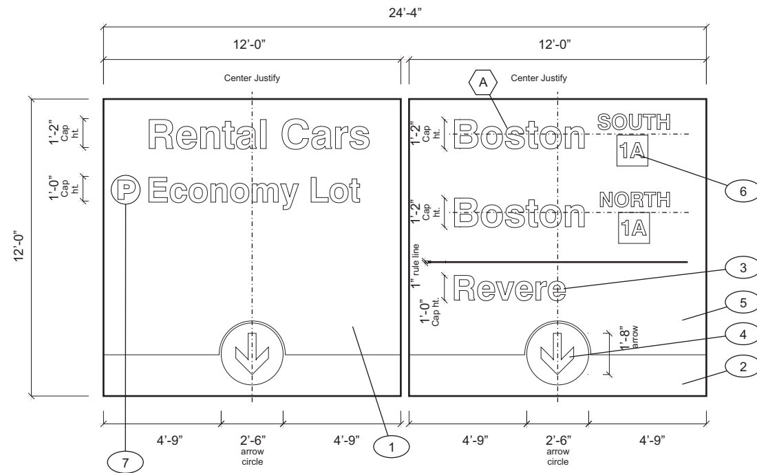
SIGN FACE ALTERNATE LAYOUT - A
