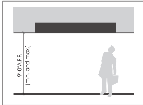
SOFFIT MOUNTED
