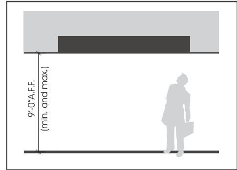
SOFFIT MOUNTED
