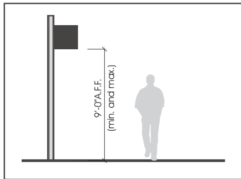
POST MOUNTED
