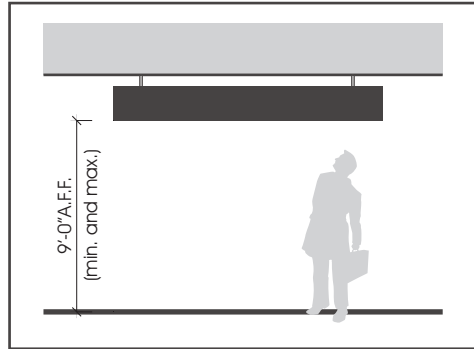
CEILING SUSPENDED
